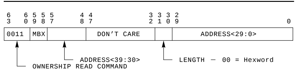
Figure 2–15 Ownership Read Command
