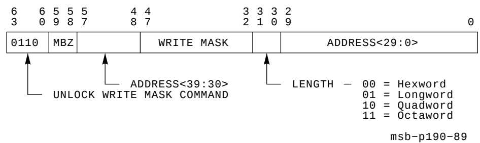
Figure 2–17 Unlock Write Mask Command
