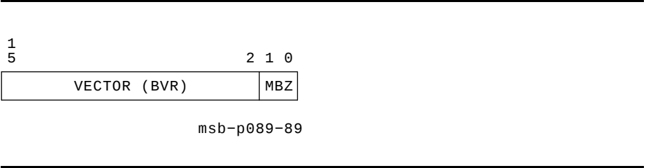
Figure 3–8 XMI Vector Format
