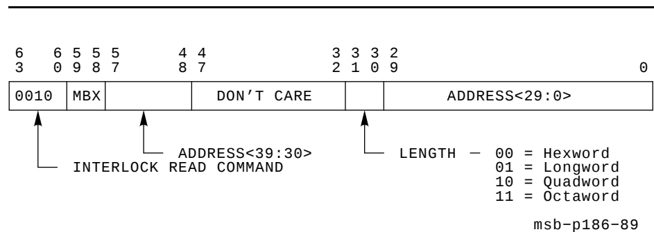
Figure 2-13 Interlock Read Command
