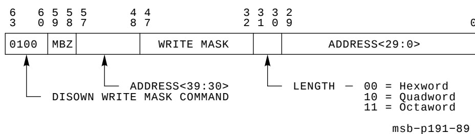
Figure 2–18 Disown Write Mask Command
