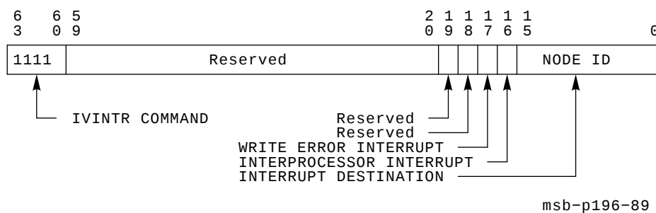
Figure 2–23 Implied Vector Interrupt Command
