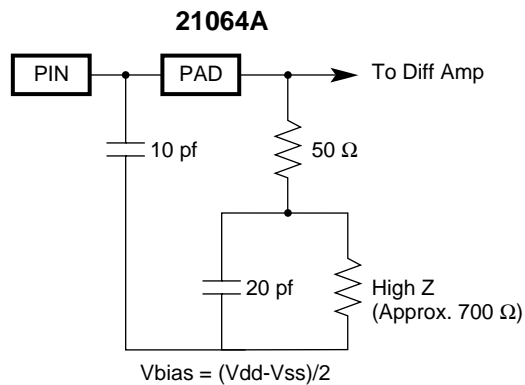
Figure 34 Clock Termination
