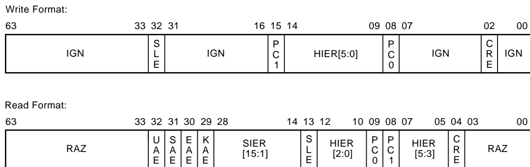
Figure 15 Hardware Interrupt Enable Register
